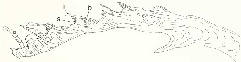
TEXT-FIG. 5. Longitudinal section through a ventral valve of Clitambonites schmidti (Pahlen) with the exterior embedded in matrix (stippled) to show a series of surface imbrications (i) underlain by a setal groove terminating proximally in a bulb (b) interpreted as containing a setal follicle. The succeeding step (s) shows fine laminae, not preserved in matrix-free shells, representing minor oscillations in the mantle edge before the growth of the succeeding imbrication. RMS Br92111; Kukruse Stage (CII); Kohtla, Estonia; \times 10 .
